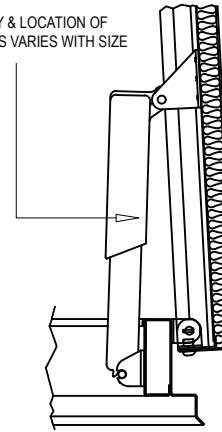
DETAIL B: SPRING DETAIL
