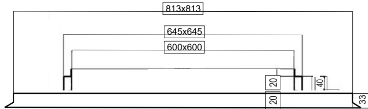
ELEVATION A 1:10
